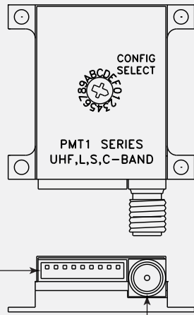
SMA Female RF Output (Connect to Antenna)
